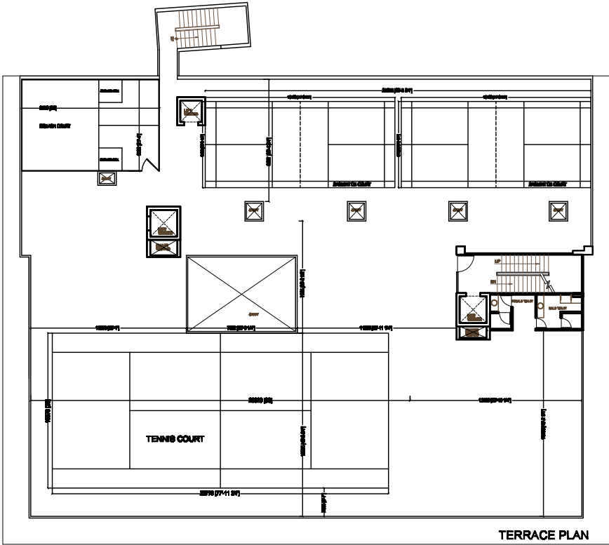
TERRACE PLAN
