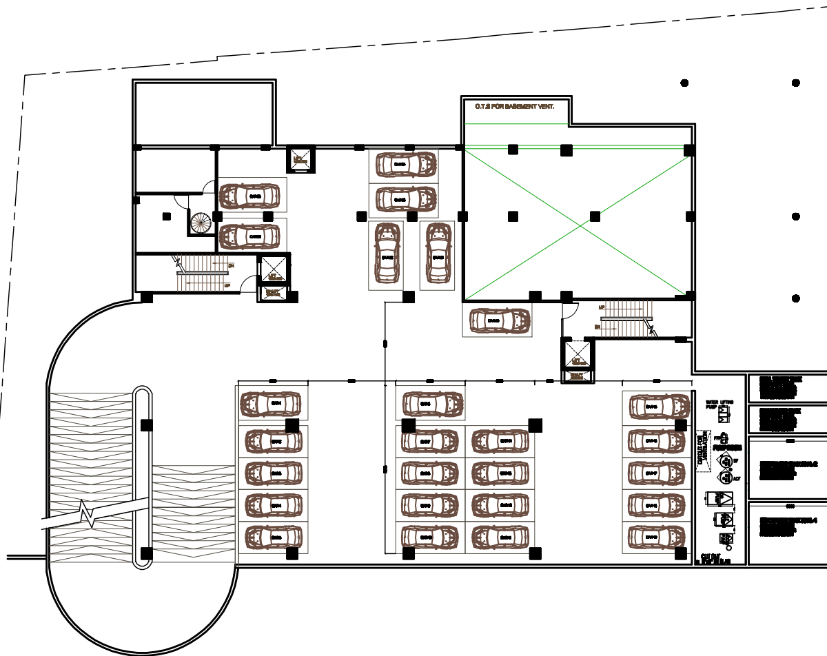
UPPER BASEMENT FLOOR PLAN
